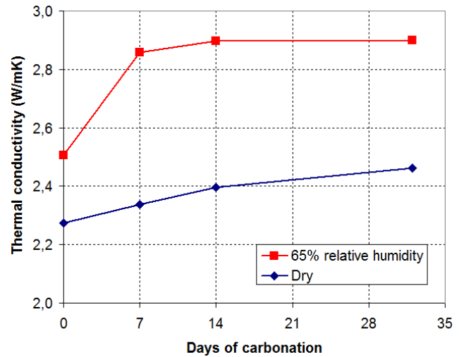
Fig. 5 Evolution of the thermal conductivity during carbonation
