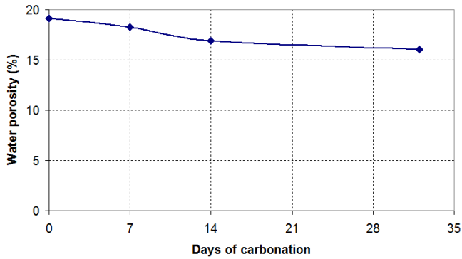
Fig. 3 Evolution of the porosity accessible to water during carbonation
