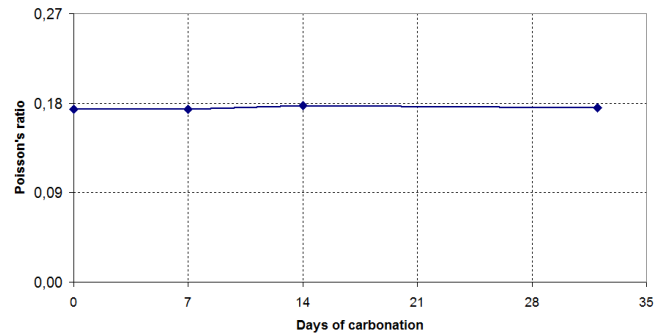
Fig. 9 Evolution of the Poisson's ratio during carbonation
