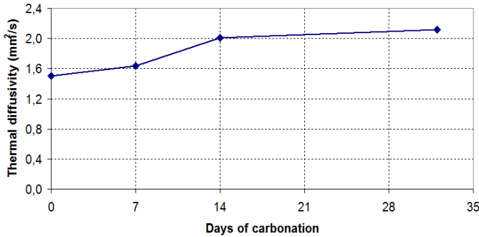
Fig. 6 Evolution of the thermal diffusivity during carbonation
