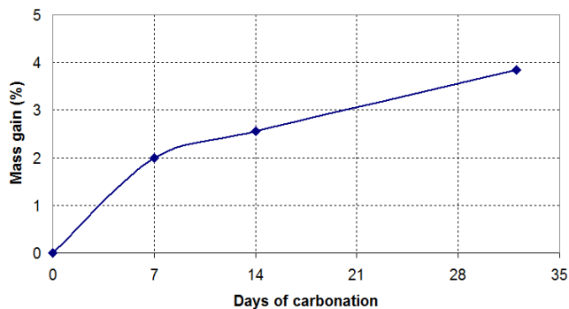
Fig. 1 Mass gain during carbonation of cement mortar
