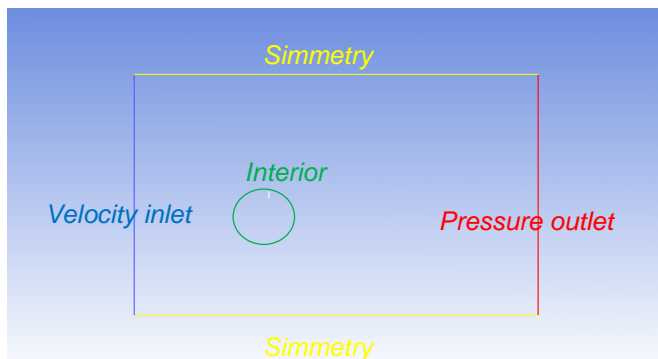
Fig. 2 Boundary conditions of the computational domain
