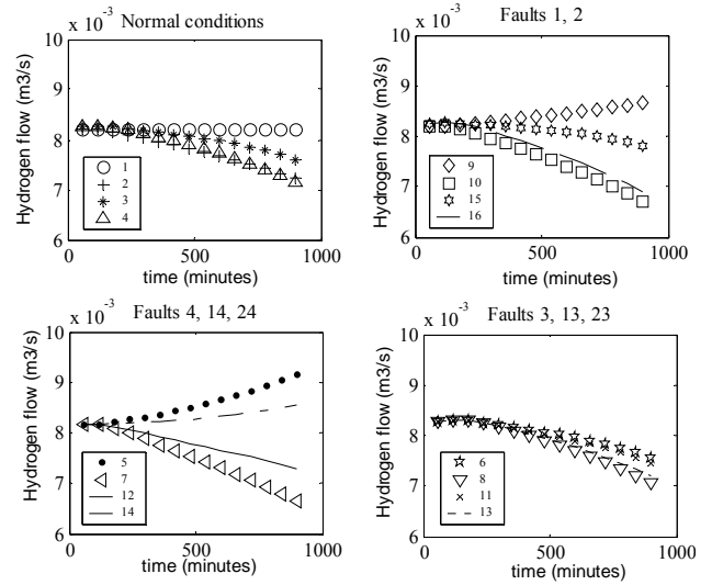
Fig. 5 Hydrogen quench flow response
