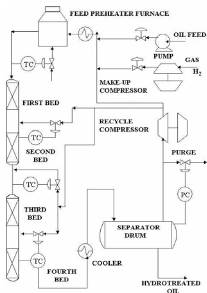
Fig. 1 Reactor and pre-heating section
