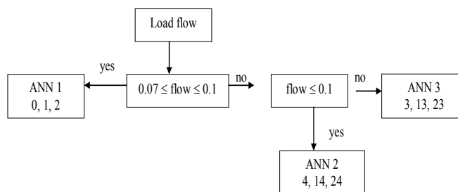
Fig. 2 Separated network approach flow-chart
