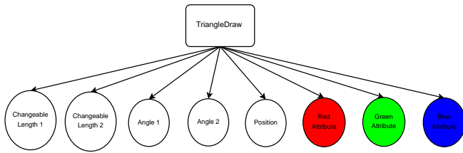
Fig. 1. The draw-triangle function with eight terminals.
