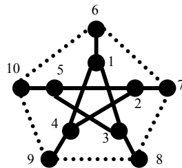
Fig. 4 Decomposition of Petersen's graph into 5-sun and C_5
