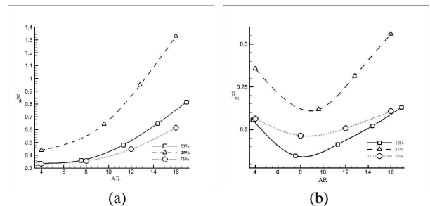
Fig. 4 Effect of porosity applying pressure (a) 490Pa; and (b) 2940Pa
