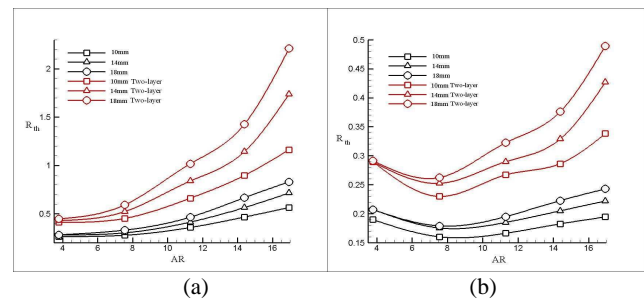
Fig. 9 Effect of microchannel length for 3mm microchannel height and two-layer with (a) 490 Pa and (b) 2940Pa
