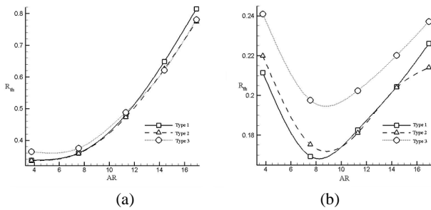
Fig. 6 Entrance effect with applying pressure difference (a) 490Pa; and (b) 2940Pa
