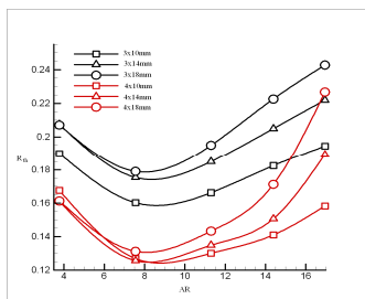
Fig. 7 Effect of microchannel length with high applying pressure difference (2940Pa) for 3mm and 4mm microchannel height
