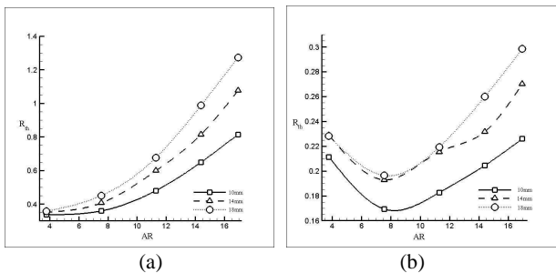
Fig. 3 Effect of microchannel length with applying pressure difference (a) 490Pa; and (b) 2940Pa
