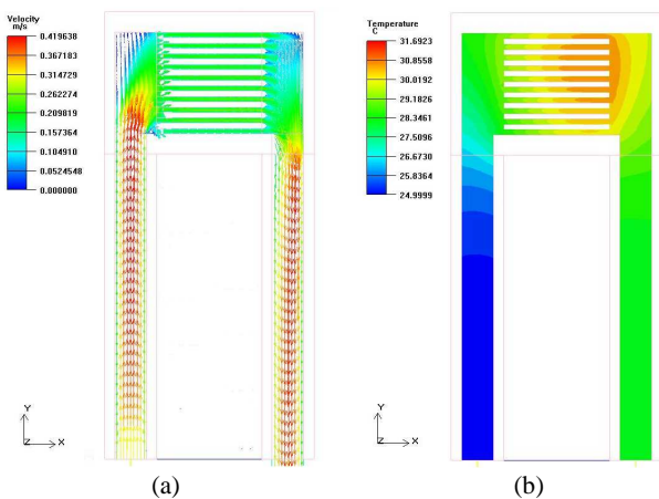
Fig. 2 (a)velocity; and (b) temperature contour diagram of the model
