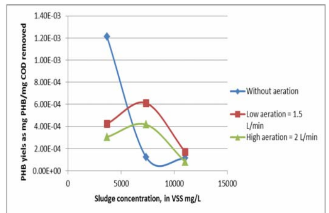
Fig.4 Effect of aeration and sludge concentration PHB yield as mgPHB/mgCOD removed
