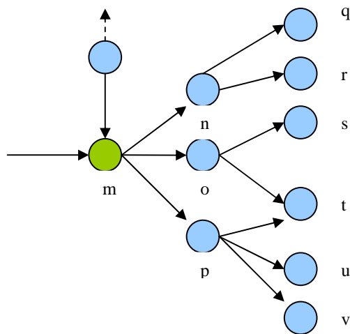
Fig. 8 A Sample Graph
