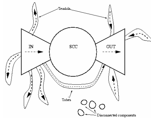
Fig. 4 Macroscopic Structure of Web [7]
