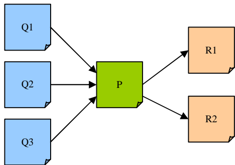
Fig. 7 Calculation of hubs and Authorities
