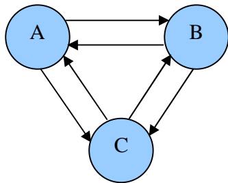
Fig. 3 A Directed Graph, G
