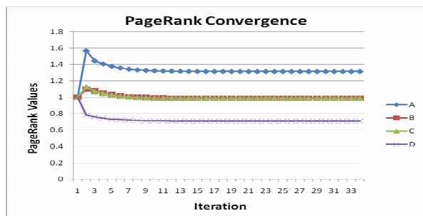
Fig. 11 (b) PageRank Convergence Chart
