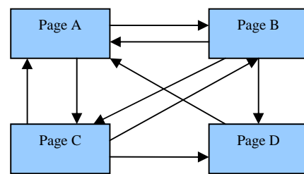
Fig. 5 Hyperlink Structure for 4 pages
