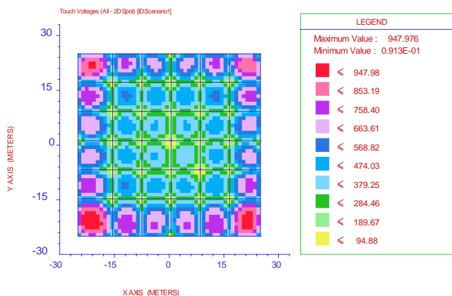
Fig. 3 Harbata Existing Touch Voltage profile
