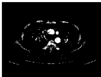
Fig. 3 Threshold image
