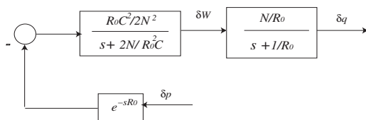
Fig. 1 Block diagram of the linearized TCP flow-control model
