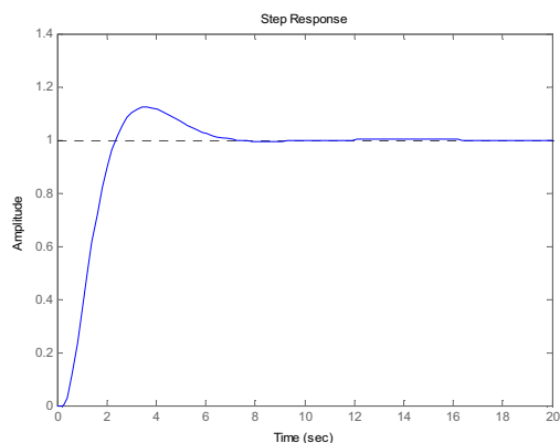
Fig. 6 Step response of the TCP/AQM closed-loop system
