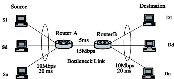
Fig. 7 Simulation of network topology
