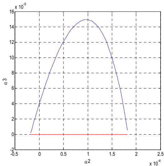
Fig. 4 Stabilizing regions in the plane (\alpha_2, \alpha_3)
