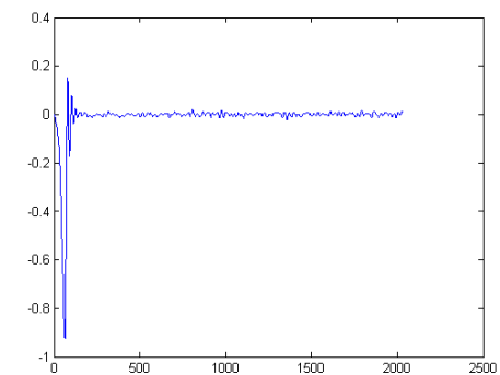
Fig. 9 i_3 response of controlled Chua's circuit with noise and perturbation using NAFT
