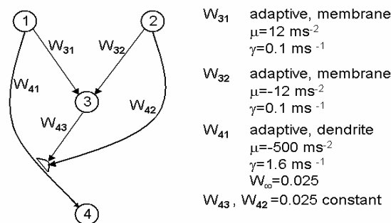
Fig. 1 The neural microcircuit
