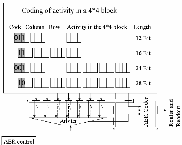
Fig. 3 Coding protocol and arbitrated pulse capture of AER
