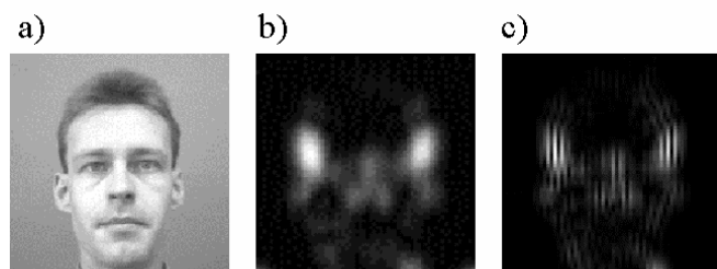
Fig. 10 Comparison of original image (a), amplitude response of an ideal Gabor image filter (b), and pulsed realization using the NPUs and router (c)
