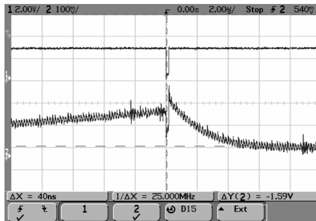
Fig. 6 Digital output (upper curve) and integrator voltage (lower curve) of the pulsing pixel cell for a single reset event
