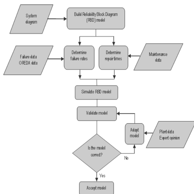
Fig. 2 Modeling approach
