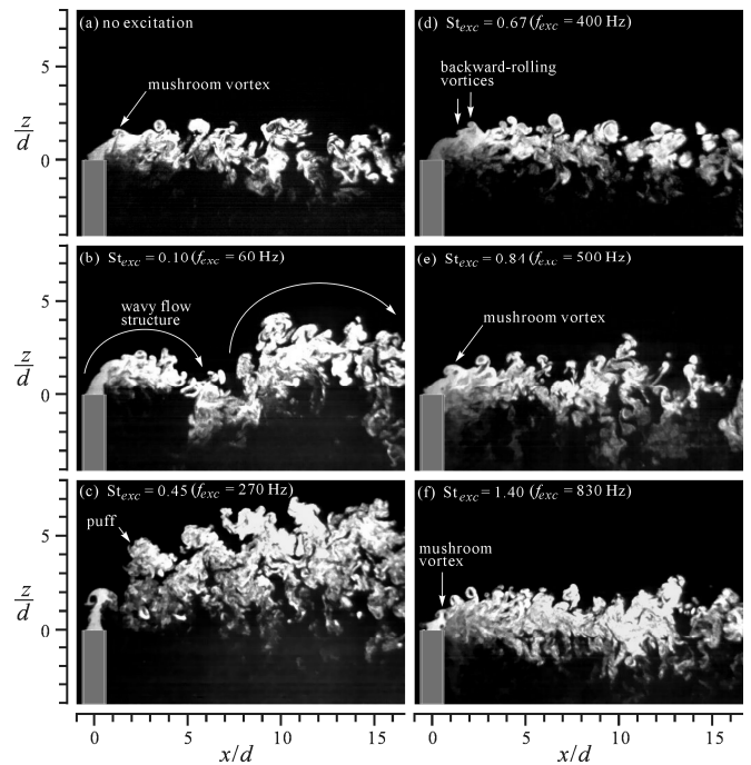
Fig. 3 Characteristic flow patterns in the median plane of the non-excited and excited transverse jet. R = 0.56 , Re_j = 1000 . Exposure time: 1/10,000 s. (a) no excitation, (b) jet oscillation mode, (c) puff mode, (d) transition mode, (e), (f) synchronized shear-layer vortices mode
