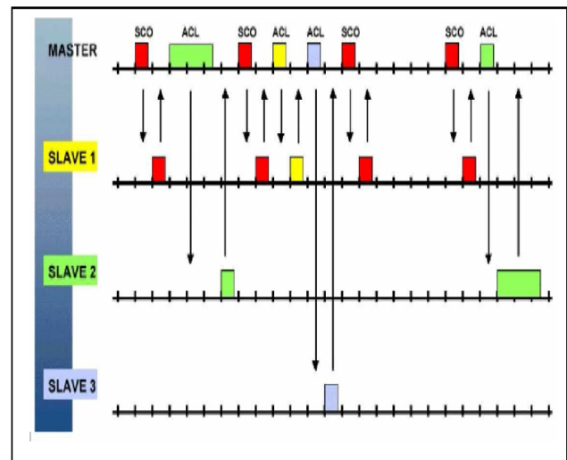
Fig. 1 Master Driven TDD Scheme
