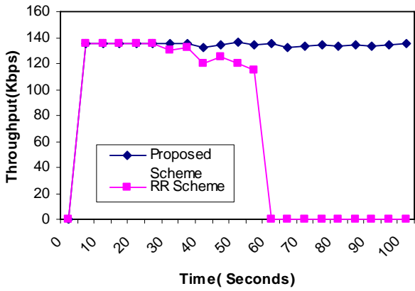
Fig. 3 Throughput of Slave 1
