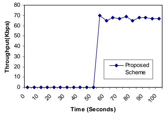
Fig. 8 Throughput of Slave 6
