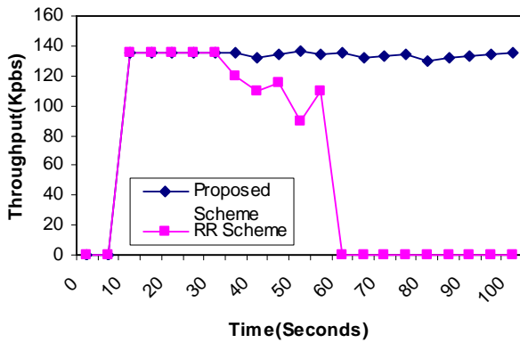
Fig. 4 Throughput of Slave 2
