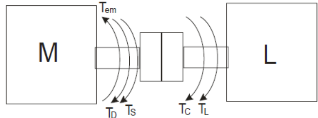
Fig. 5 Mechanical system with torques
