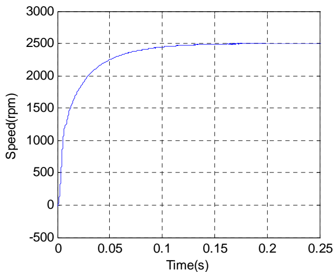
Fig. 6 Waveform of rotary speed
