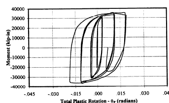
Fig. 1 Hysteretic behavior of test (UTA-1R) [10]
