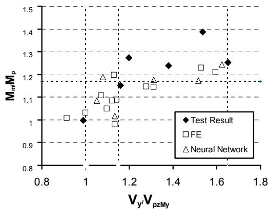
Fig. 15 M_m / M_p ratio versus (V_y/V_{pzMMy})
