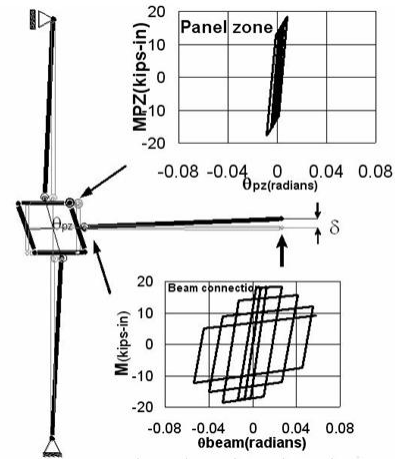
Fig. 24 Analytical model Specimen RN2
