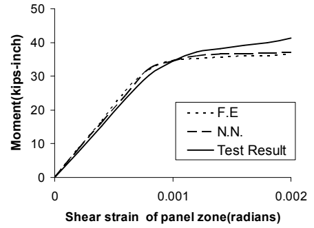
Fig 7 Result of FE and N.N. and experimental results for one sided haunch for specimen UCB-R2 and UCSD-1R
