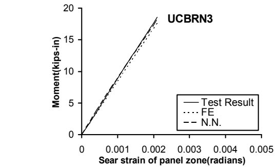
Fig. 8 Result of FE and N.N. and experimental results for double sided haunch for specimen UTA-3R and UCBRN3
