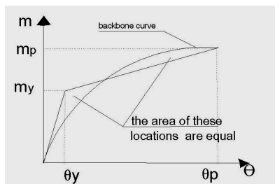
Fig. 10 Typical moment-rotation curve of connection and its reference moment
