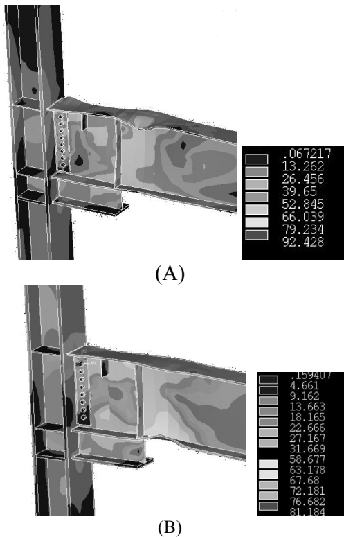
Fig. 18 Von Misses stress distribution of model ucSD-6 (loading step 15and 16)
