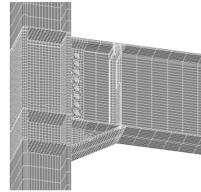
Fig. 12 FE model of specimen (ucsd-3R)
