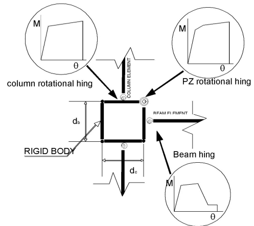
Fig. 23 PZ modeling used in this study
