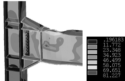
Fig. 16 Von Misses distribution (UCB RN3)
