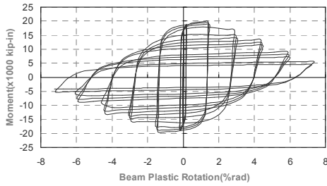
Fig. 4 Hysteretic behavior of numerical model (UCB-RN3)
