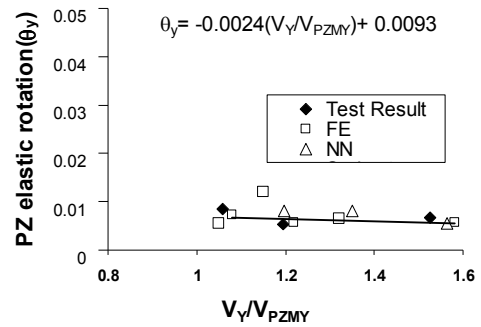
Fig. 20 PZ elastic rotation versus (V_y/V_{pzMMy})
