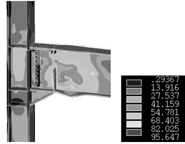
Figure 11 Von Mises distribution (ucscd-3R)
