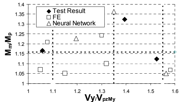
Fig. 22 M_m / M_p ratio versus (V_y/V_{pzMMy})
