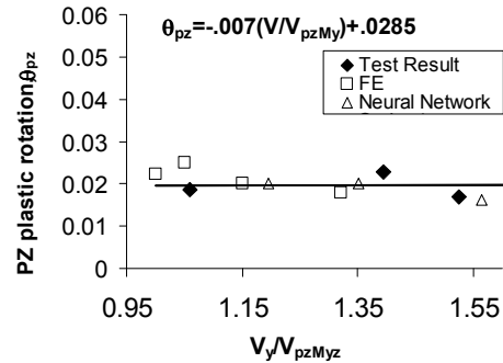
Fig. 21 PZ plastic rotation versus (V_y/V_{pzMMy})
