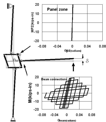
Fig. 25 Analytical model Specimen UCB-RN3
