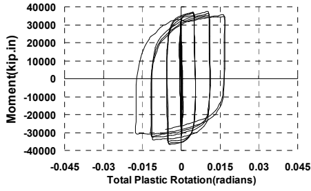
Fig. 2 Hysteretic behavior of numerical model (UTA-1R)
