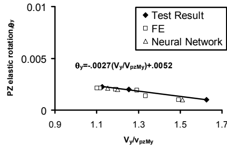
Fig. 17 PZ elastic rotation versus (V_y/V_{pzMMy})
