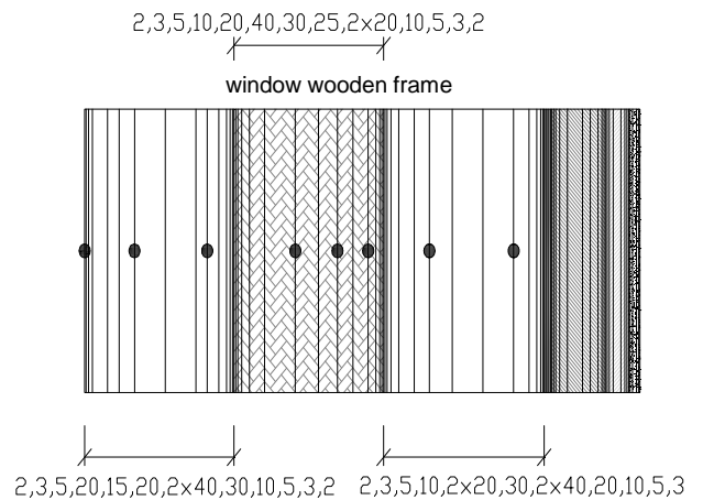
Fig. 10 Sensors placing and computer generated mesh, section B-B'
