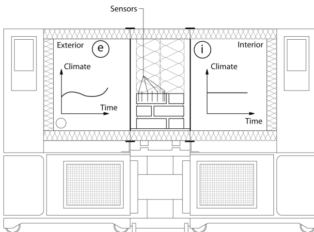
Fig. 1 Scheme of the climatic chamber system
