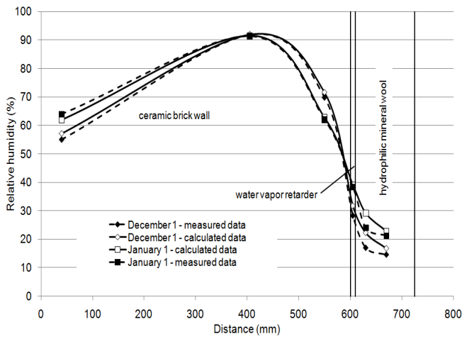
Fig. 11 Relative humidity profiles, section A-A'
