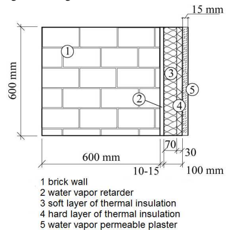
Fig. 2 Scheme of the tested building envelope
