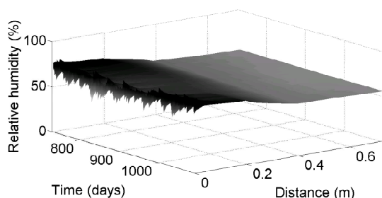
Fig. 16 Relative humidity distribution in the studied structure during 3 rd year of simulation, section B-B'
