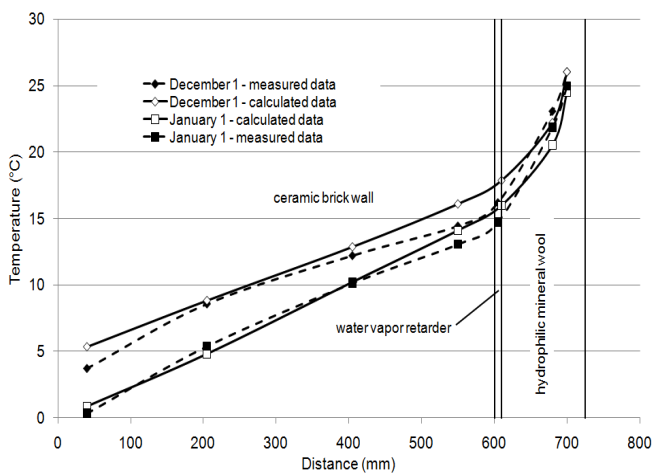
Fig. 12 Temperature profiles, section A-A'
