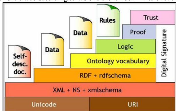
Fig. 1 Stratification of Semantic Web technologies
