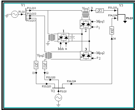
Fig. 2 Multi-machines system with the new developed UPFC
