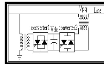
Fig. 1 A block diagram of a UPFC
