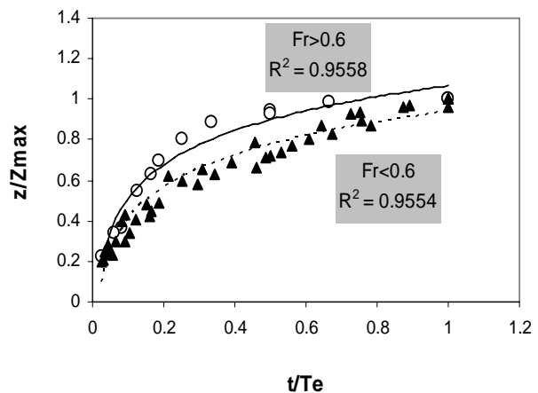
Fig. 3 Variation of scour depth against time
