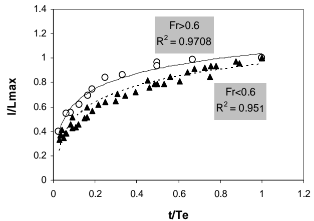
Fig. 7 Variation of scour length against time
