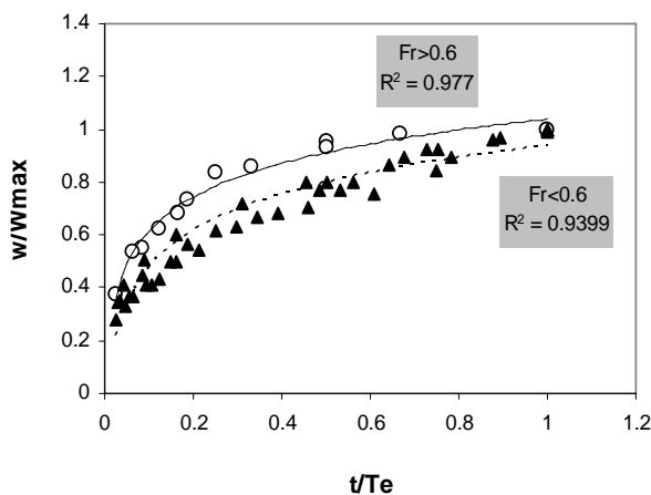
Fig. 6 Variation of scour width against time
