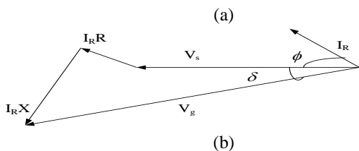
Fig. 1 (a). Utility network with wind DG system (b) phasor diagram
