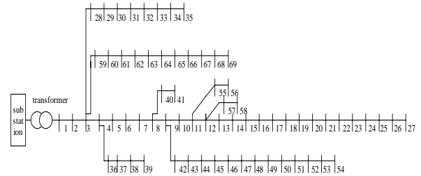
Fig. 3 Radial distribution feeder with 69 buses
