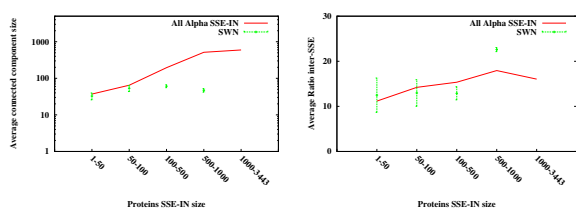
Fig. 9. Average connected component size (left) and shortcut ratio (right) as a function of protein SSE-In size.
