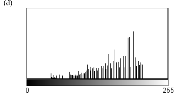
Fig. 6 Histogram for the test 03 - a) 20 N, b) 50 N, c) 140 N and d) 300N
