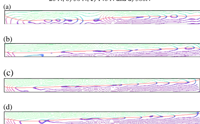
Fig. 8 Isochromatic lines representation for the testing specimen 2. a) 20 N, b) 50 N, c) 140 N and d) 300N
