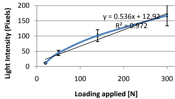
Fig. 3 Average pixel light intensity versus loading
