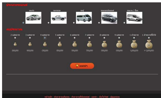
Fig. 6 Feature selection
