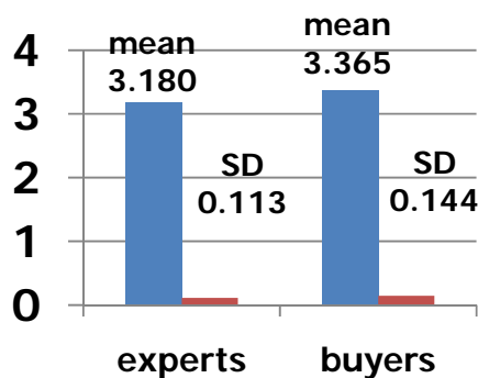
Fig. 11 Rating comparison
