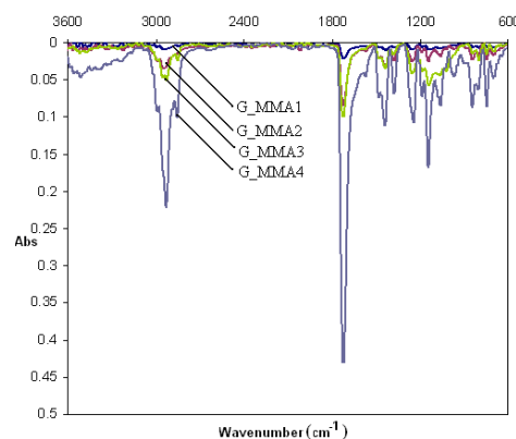
Fig. 2 ATR-FTIR spectra of the copolymers (G_MMAx)
