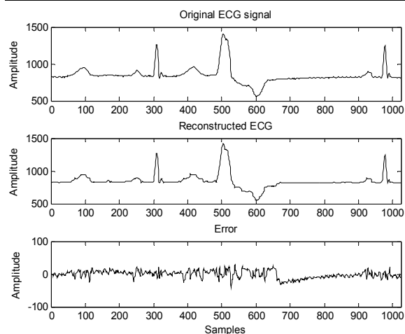
Fig. 7 ECG 119 with CR= 45.83, PRD=1.31 Top figure is original signal, the middle is reconstructed signal and bottom signal is error
