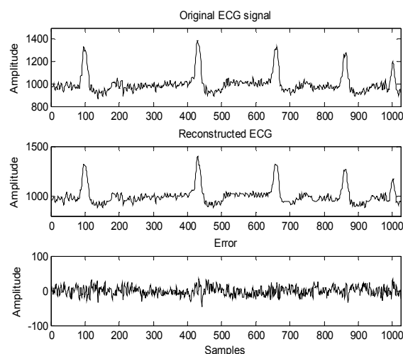
Fig. 10 ECG 203 with CR= 48.38, PRD= 1.18 Top figure is original signal, the middle is reconstructed signal and bottom signal is error
