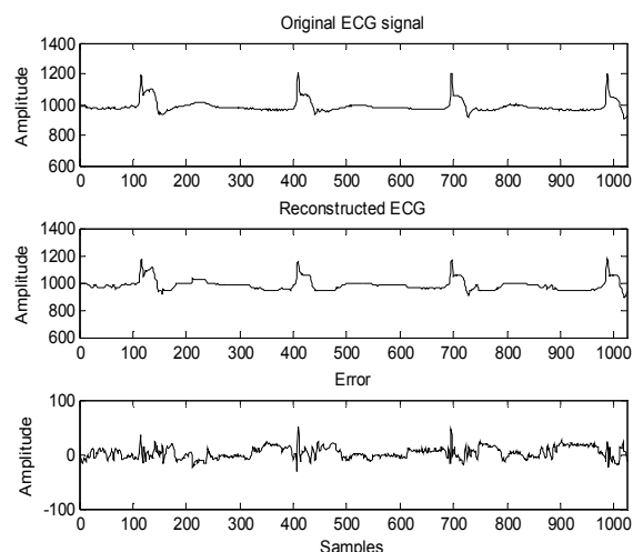
Fig. 9 ECG 102 with CR=46.41, PRD= 1.10 Top figure is original signal, the middle is reconstructed signal and bottom signal is error
