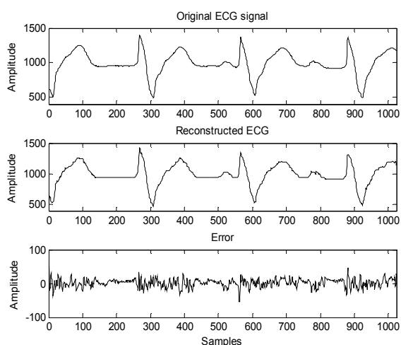
Fig. 8 ECG 107 with CR= 48.15, PRD= 1.18 Top figure is original signal, the middle is reconstructed signal and bottom signal is error
