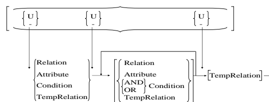
Fig. 1 Structure of free-form query language (Note: { } denotes either/or, [ ] denotes optional)
