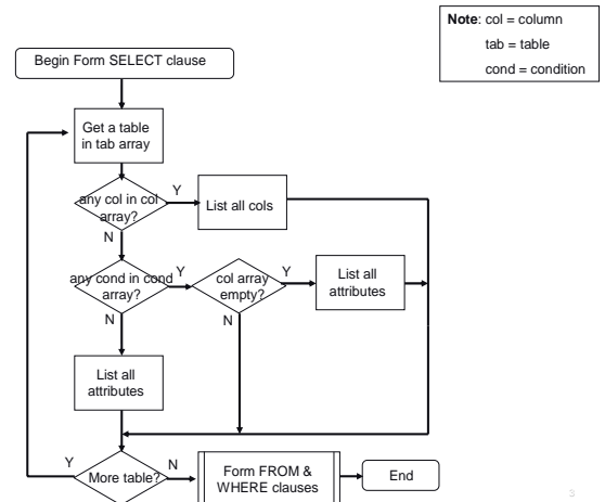
Fig. 4 Flowchart for Form SELECT clause module
