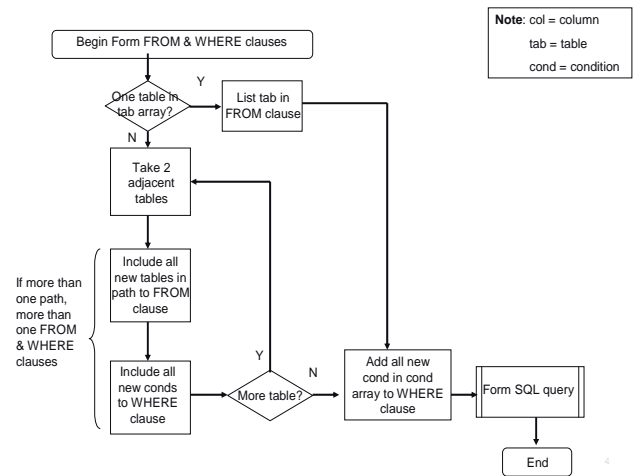
Fig. 5 Flowchart for Form FROM & WHERE clauses module
