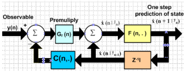
Fig. 6 Extended Kalman filter-one step predictor
