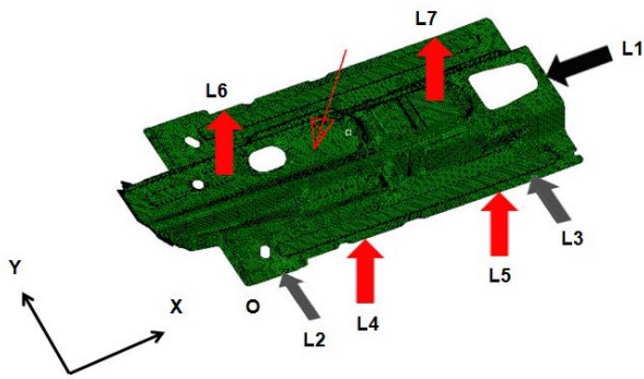
Fig. 4 Finite element model of central tunnel
