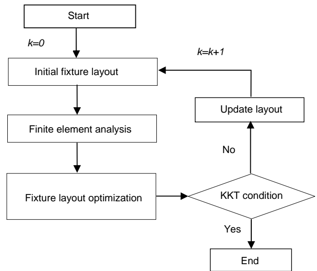
Fig. 1 Flow chart for fixture layout optimization
