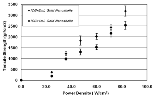
Fig. 2 Variation of tissue tensile strength with laser power densities at different solder combinations
