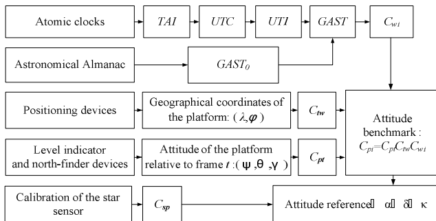
Fig. 5 The whole process to get the reference attitude based on benchmark
