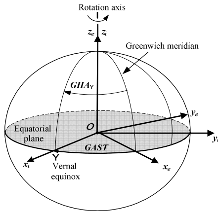
Fig. 2 The Greenwich hour angle of the equinox
