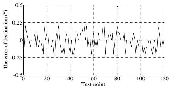
Fig. 7 The error curve of \delta
