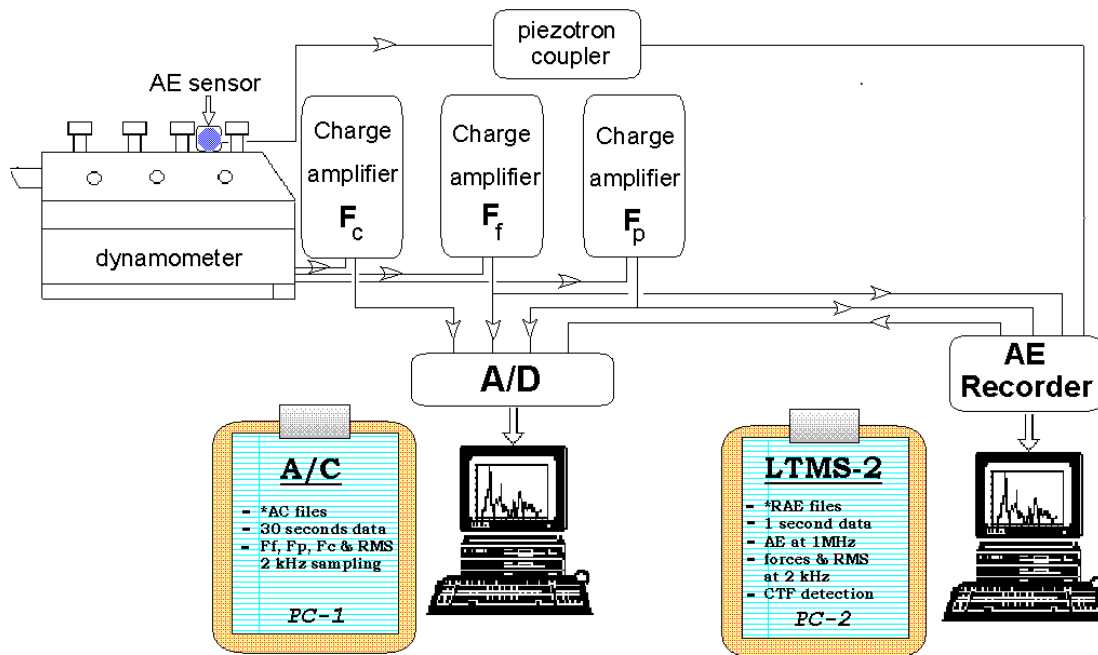
Fig. 1 Tool failure monitoring apparatus set-up
