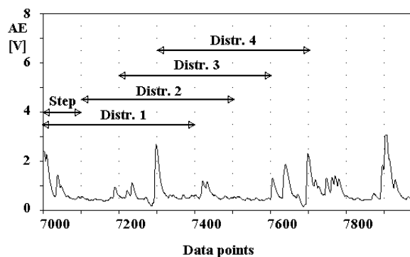
Fig. 4 Overlapping distributions
