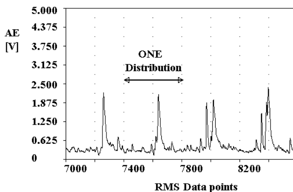
Fig. 3 Arrangement of number of data points taken in each distribution in the case of interrupted cutting
