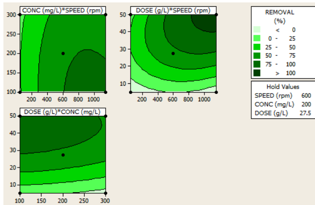
Fig. 4 Contour plots of dye removal efficiency
