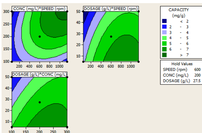
Fig. 5 Contour plots of dye capacity uptake by PSAC
