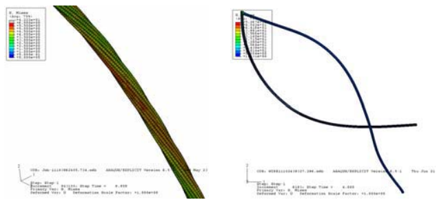
(a) Stresses distribution (b) Maximum deflection of cable bundle Fig. 7 Non linear large-deflection analysis with stress distribution and maximum deflection with before and after case 5 (ABAQUS)
