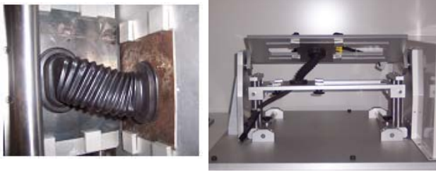
(b) Lift gate setting for W/H simulation Fig. 5 3D model simulation for slam tester and W/H setting
