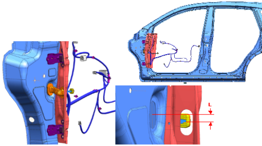
Fig. 2 Door structure and wiring harness(W/H) system
