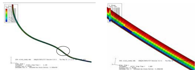
Fig. 8 Von- Mises Stresses in wire cable (7 No of cable, case 2)
