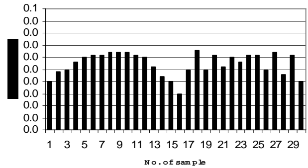
Fig. 2 Graph of Sulfur Dioxide observations
