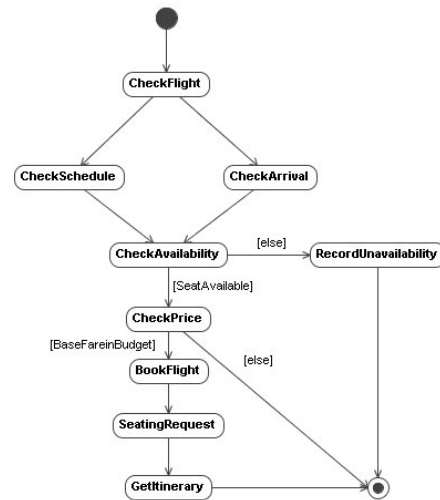
Fig. 4 Business process of flight reservation domain
