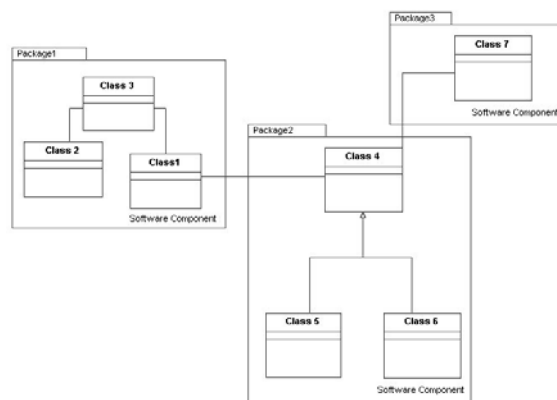
Fig. 1 Class model designed with three software components
