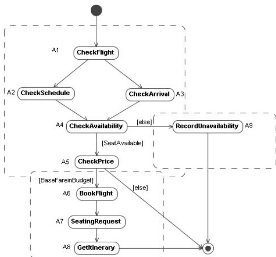
Fig. 5 A design with three process components
