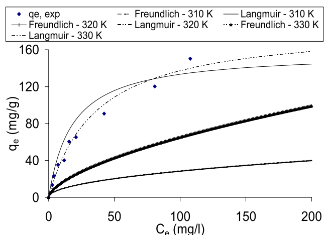
Fig. 8 Non-linear plots of Freundlich and Langmuir isotherm
