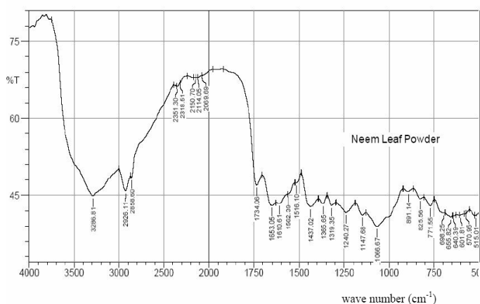
Fig. 2 FT-IR spectra of NLP
