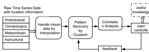
Fig. 2 A simplified architecture for the system
