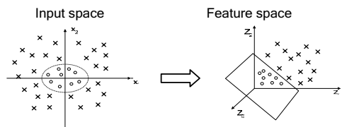
Fig. 3 Mapping nonlinear data to a higher dimensional feature space where a linear separating hyperplane can be found, eg, via the nonlinear map \Phi(x) = (z_1, z_2, z_3) = ([x]_1^2, [x]_2^2, \sqrt{2}[x]_1[x]_2)
