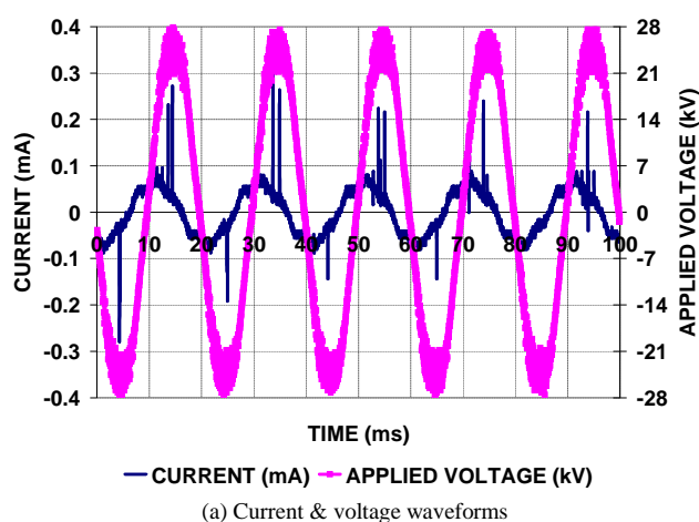
(a) Current & voltage waveforms
