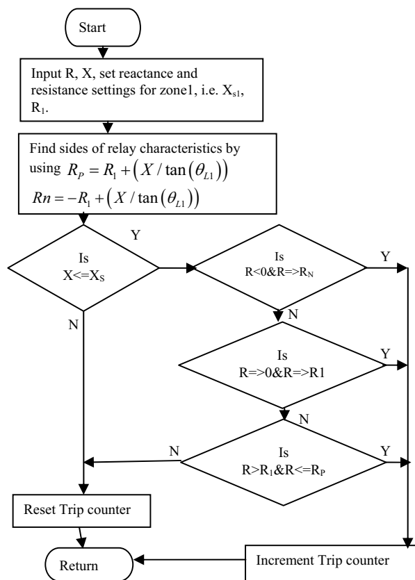
Fig. 7. Quadrilateral Relay Logic for Zone1.
