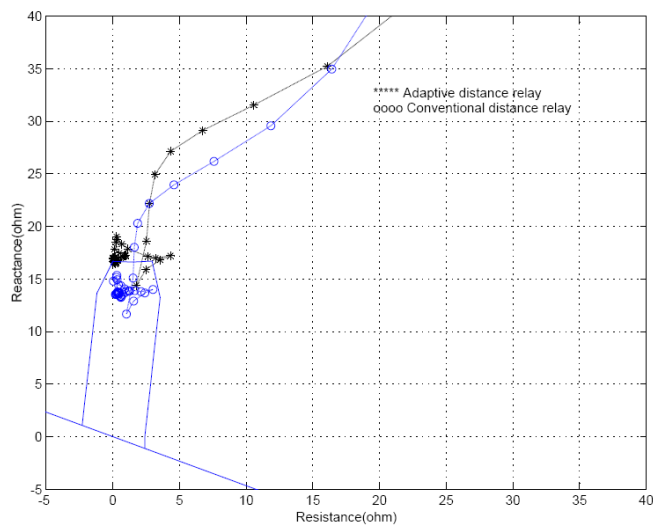
Fig. 8. R-X Diagrams of Adaptive and Conventional Relay for the case (a.6).
