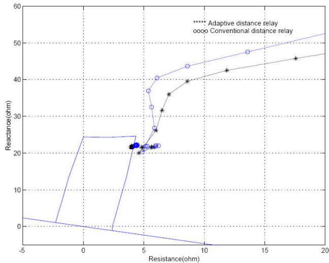
Fig. 10. R-X Diagrams of Adaptive and Conventional Relay for the case (b.2).
