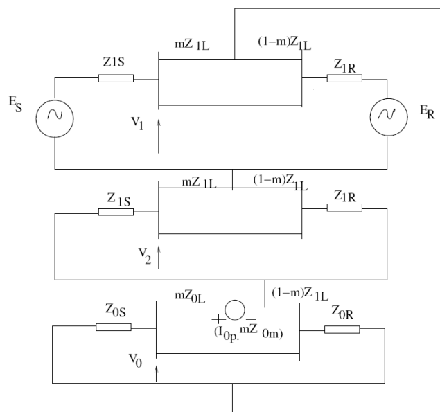
Fig. 3. Phase-To Ground Fault in One of Two Parallel Lines with Zero Sequence Mutual Coupling.
