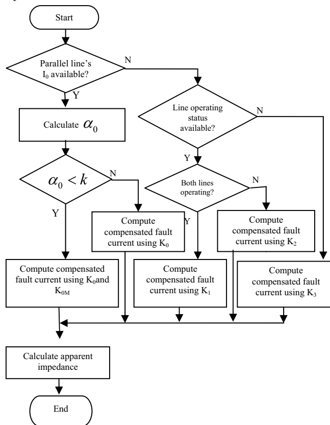
Fig.5. Adaptive Distance Protection logic Scheme Flow
