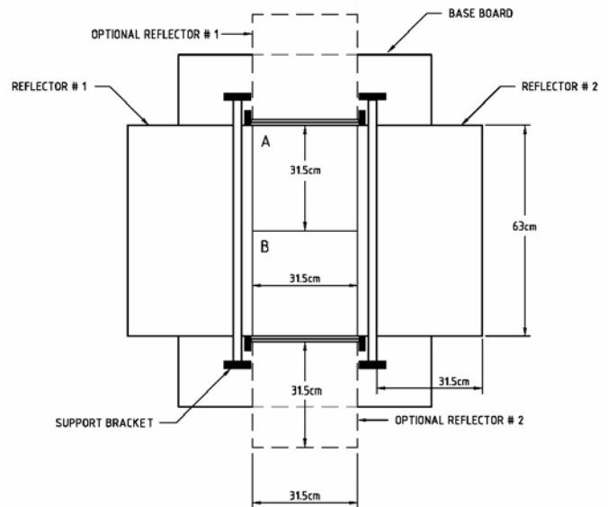
Fig. 4 Solar Intensifier Unit with 4 reflectors
