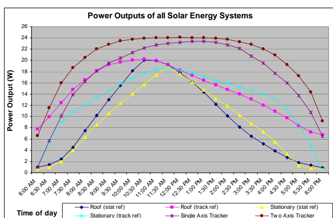
Fig. 8 Power outputs of all solar energy systems
