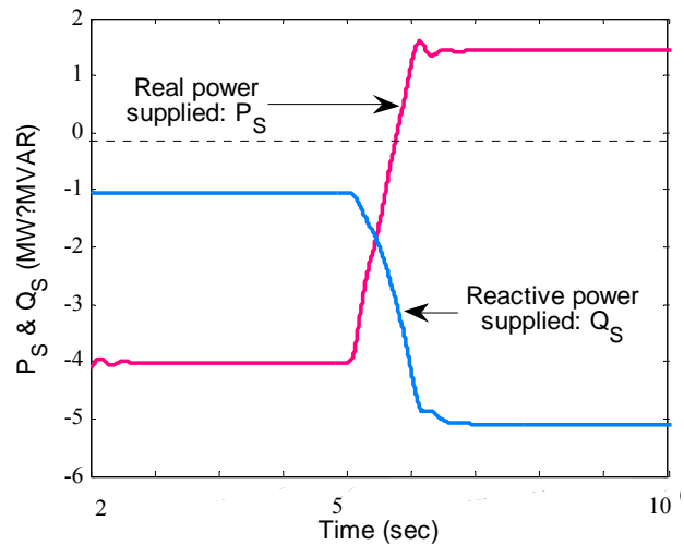
Fig. 9 Active and reactive power supplied by WTIGs to the grid for linear change of wind speed
