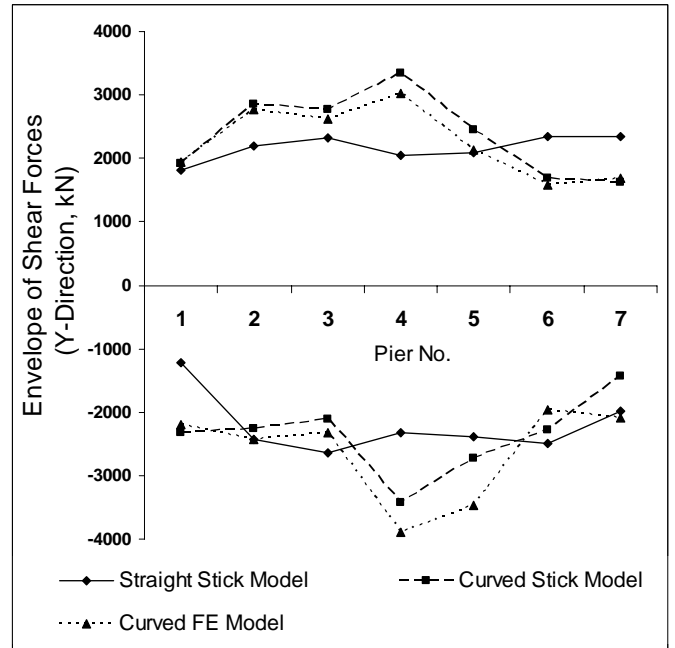
Fig. 12 Comparison of column shear forces in transverse direction at bottom
