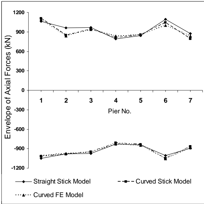
Fig. 10 Comparison of column axial forces at bottom
