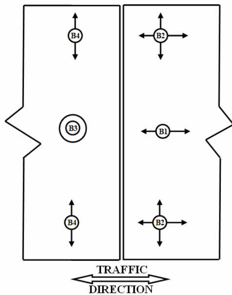
Fig. 3 Arrangement of bearings
