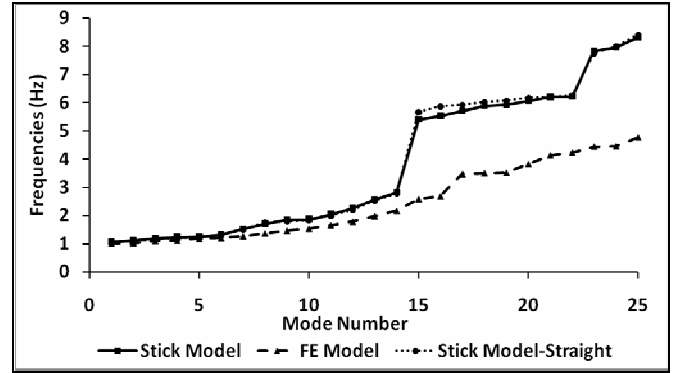
Fig. 9 Comparison of natural frequencies
