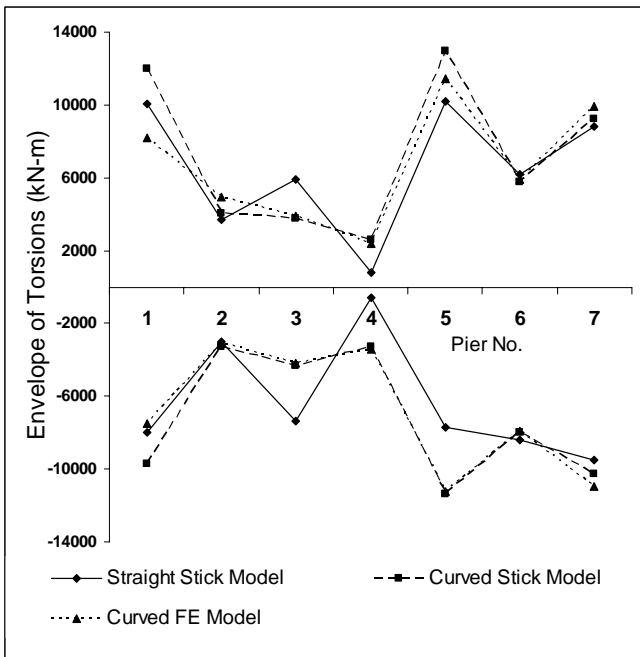
Fig. 15 Comparison of column torsion at bottom
