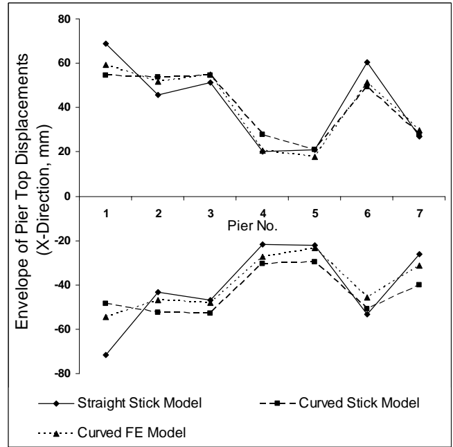
Fig. 16 Comparison of pier top X-displacement
