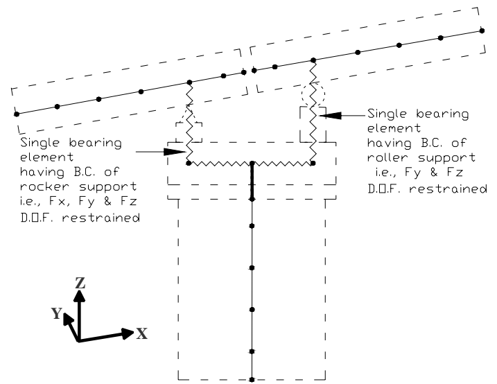
Fig. 5 Conventional stick model expansion joint
