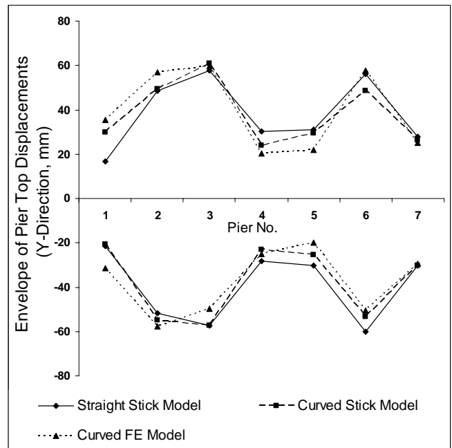
Fig. 17 Comparison of pier top X-displacement
