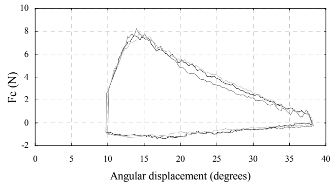
Fig. 6 Repeatability analysis for a given sample
