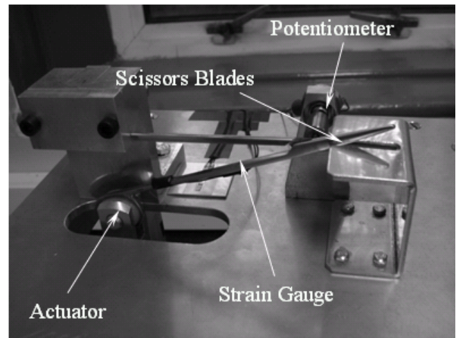
Fig. 1 Scissor cutting unit
