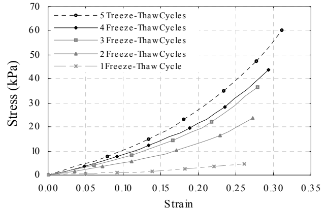
Fig. 5 Stress strain data for PVA samples
