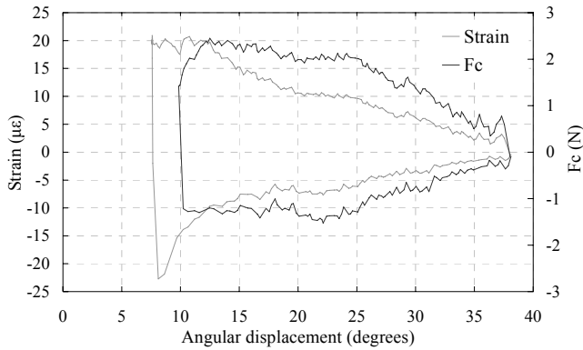
Fig. 4 Force and strain comparison
