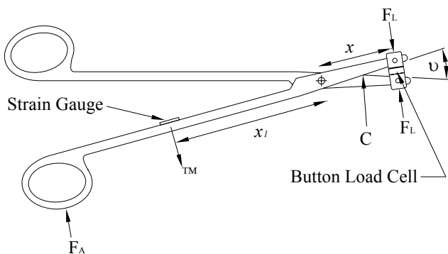
Fig. 3 Scissor geometry
