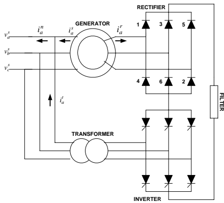
Fig. 3 Basic Power Circuit of a DOIG
