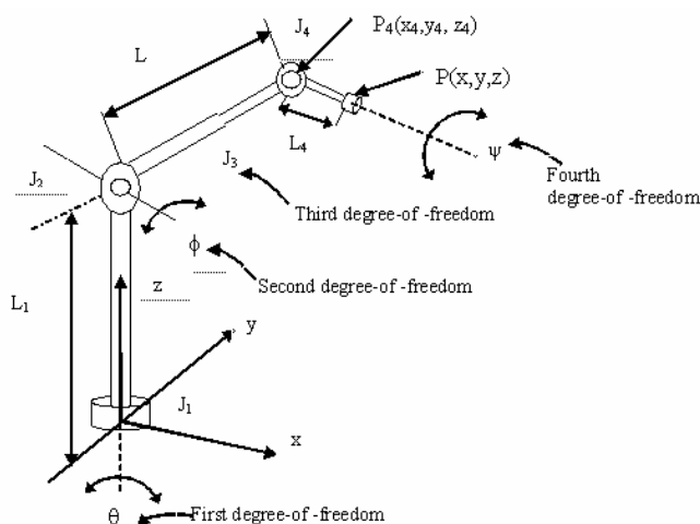
Fig. 1. Four degree-of-freedom manipulator
