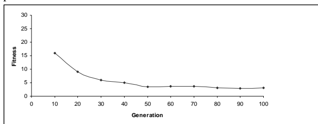
Fig. 3. Fitness versus generations graph
