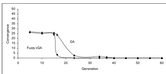
Fig. 4. Convergence versus generation graph
