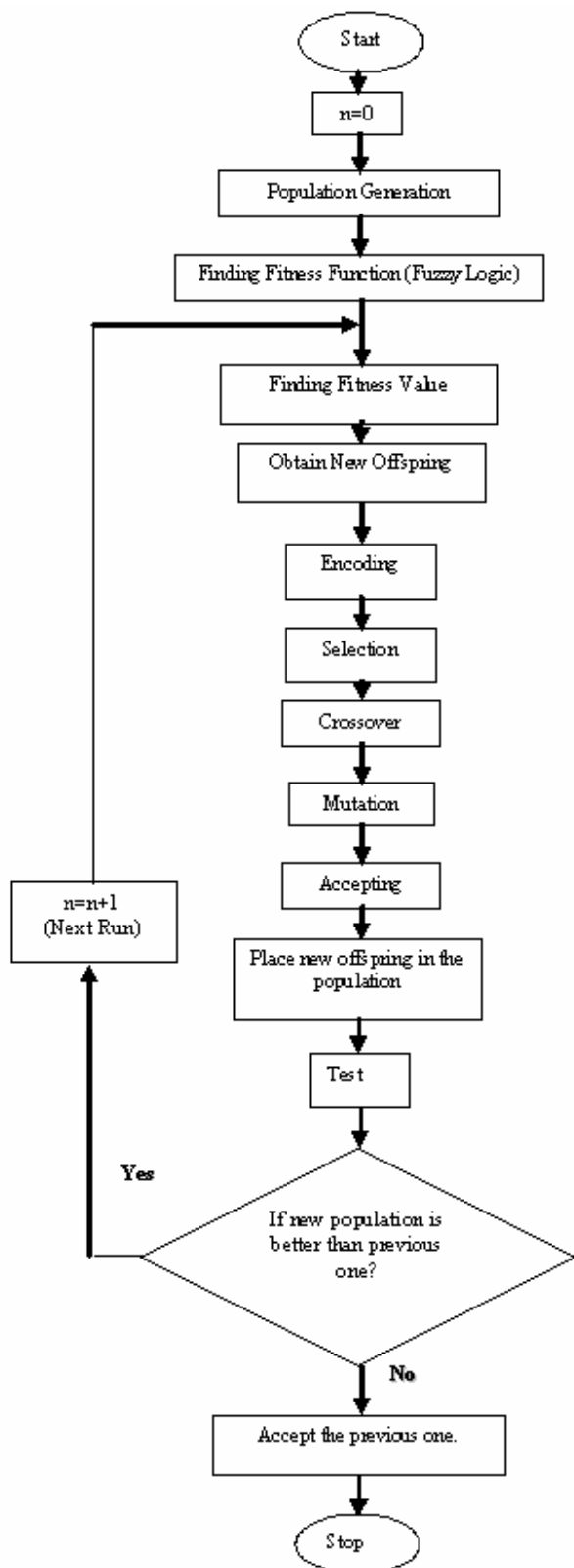
Fig. 2. Flowchart Using Genetic Algorithm
