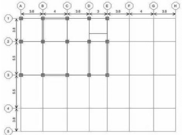
Fig. 7 Seventeenth to twentieth Floor Plan (ST 17 to 20)
