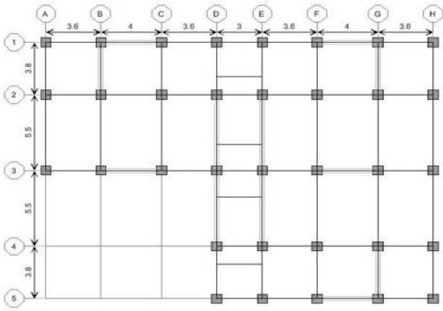
Fig. 4 Sixth to tenth Floor Plan (ST 6 to 10)
