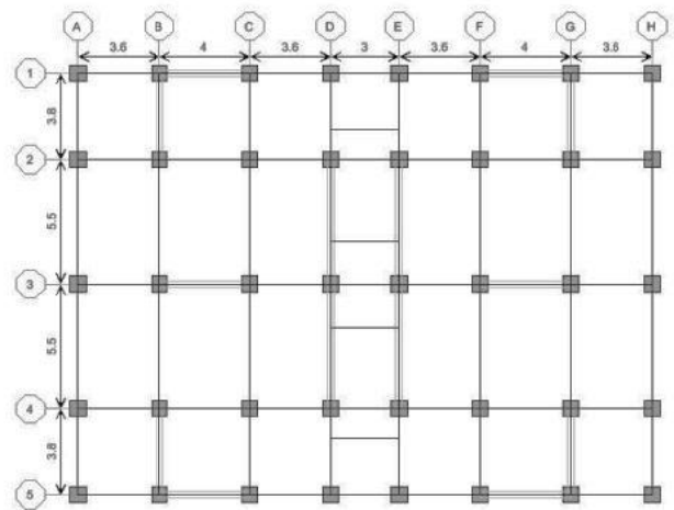
Fig. 3 First to fifth Floor Plan (ST 1 to 5)
