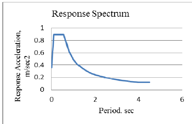
Fig. 1 Response spectrum standard of the model
