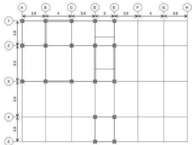
Fig. 5 Eleventh to fifteenth Floor Plan (ST 11 to 15)
