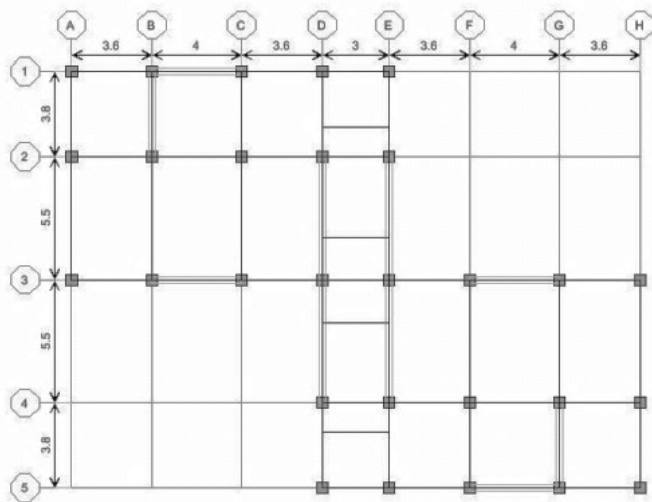
Fig. 4 Sixth to tenth Floor Plan (ST 6 to 10)
