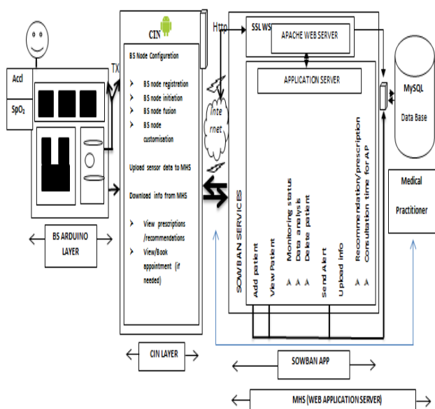
Fig. 1 SOWBAN Architecture
